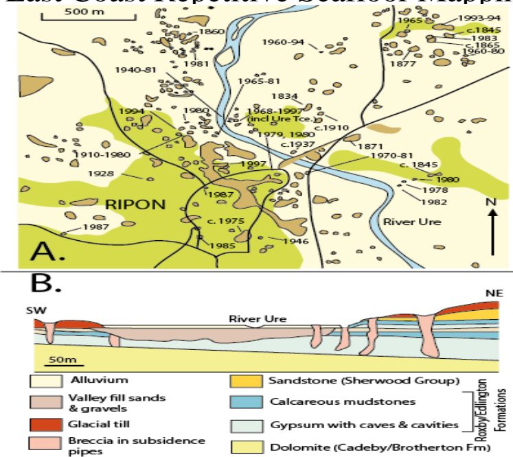
Figure 4. Ripon karst, Yorkshire, UK. A) Surface distribution of karst features (shaded brown) and time of formation, where known, of various subsidence features and collapse dolines surfacing in and around the town of Ripon. Urban areas are shaded green. B) Idealised geological cross section (after Cooper and Waltham, 1999; Jones and Cooper, 2005).
