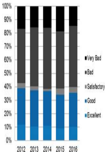
Groundwater Quality Deterioration 2012-2016
