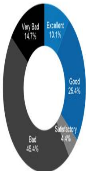
2016 Overall Groundwater Quality
